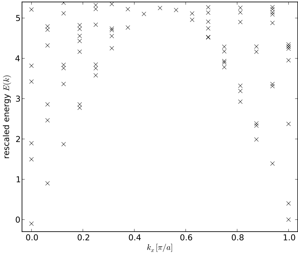
Galois conjugate of golden chain ( J=1, L=32 )
