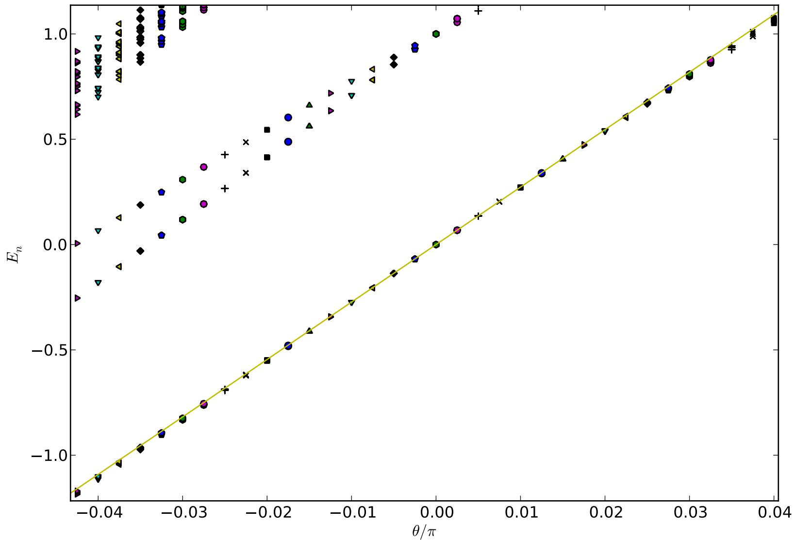
Fibonacci anyons on 2x2 honeycomb
