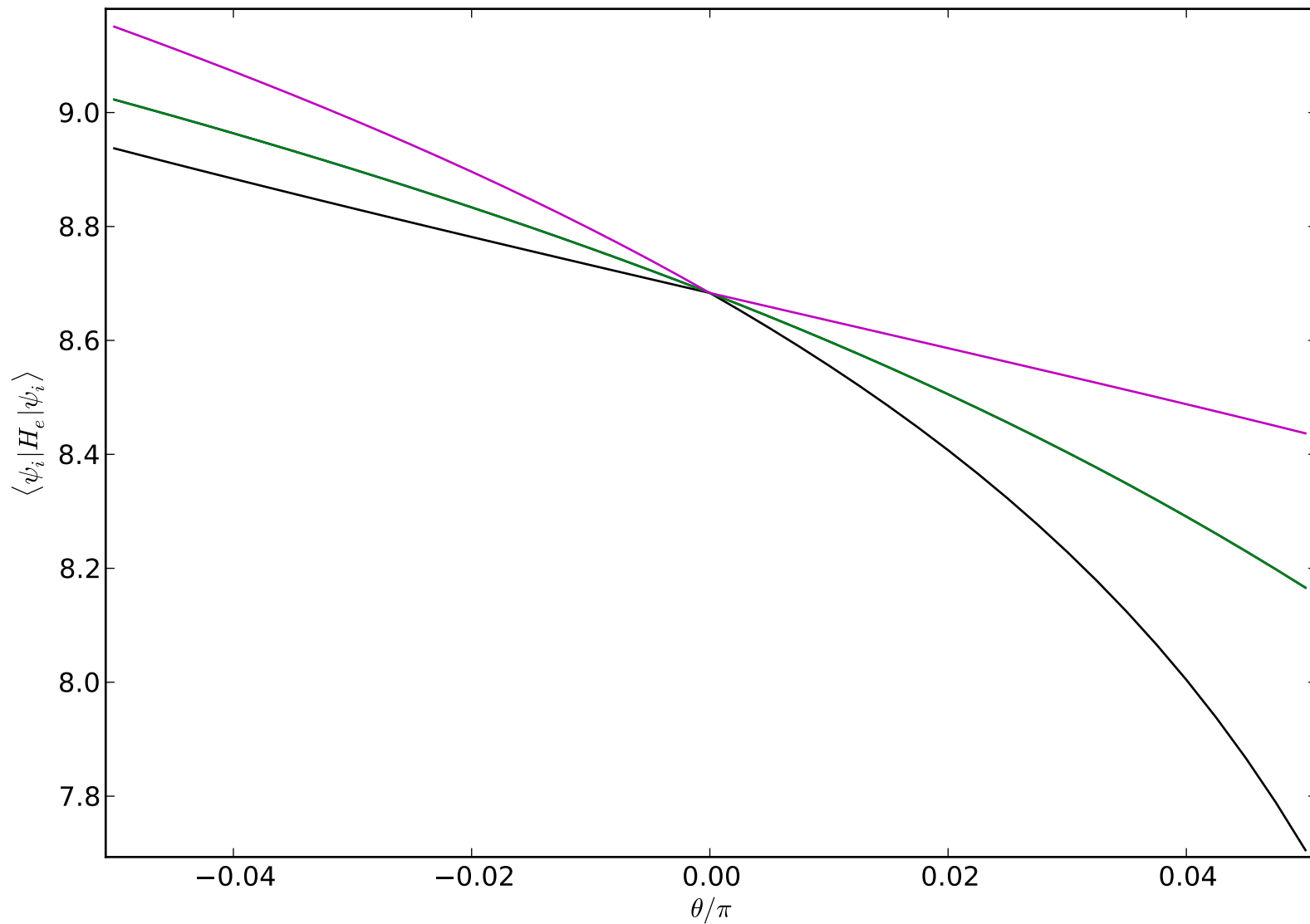
Fibonacci anyons on 2x2 honeycomb: string tension
