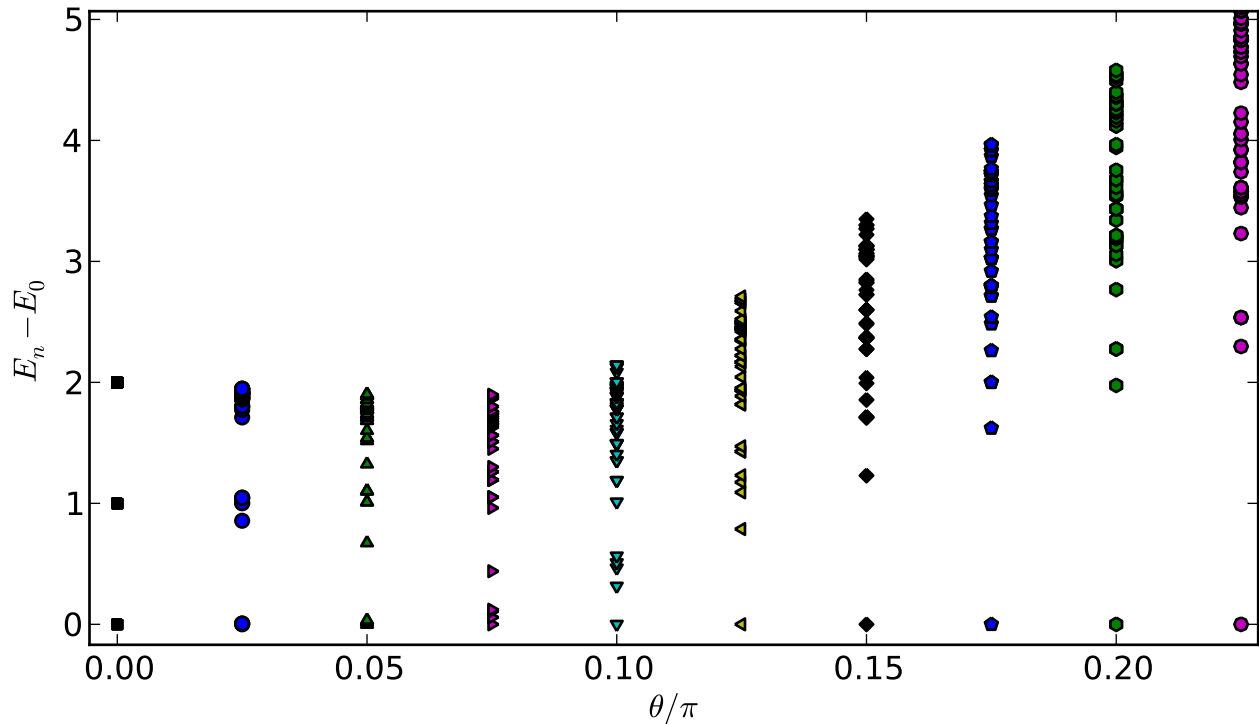
Spectrum of Fibonacci anyons on 3x2 honeycomb lattice
