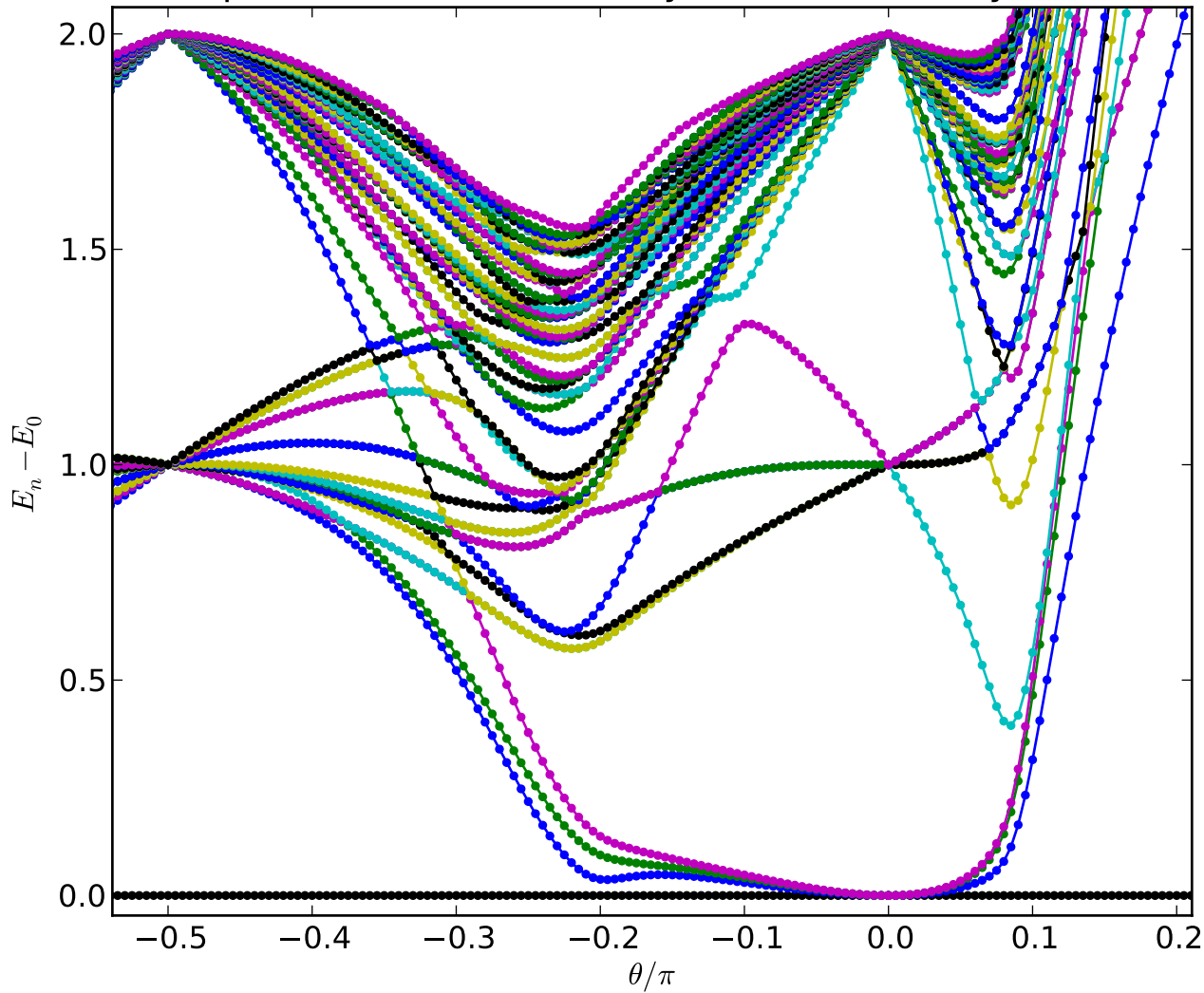
Spectrum of Fibonacci anyons on 3x2 honeycomb
