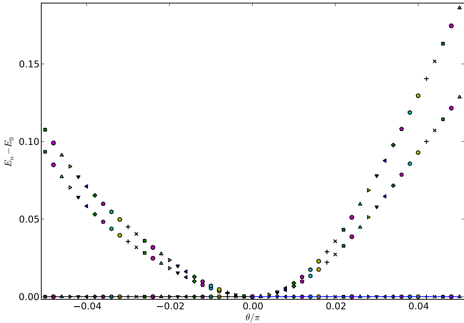
Galois conjugate on 2x2 honeycomb
