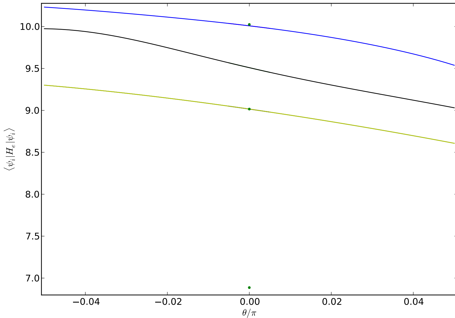
Galois conjugate on 2x2 honeycomb: string tension
