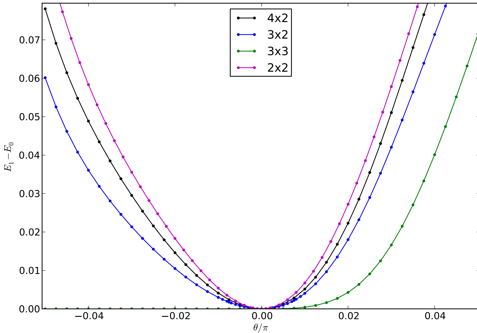
Galois conjugate on honeycomb: 1st excited state
