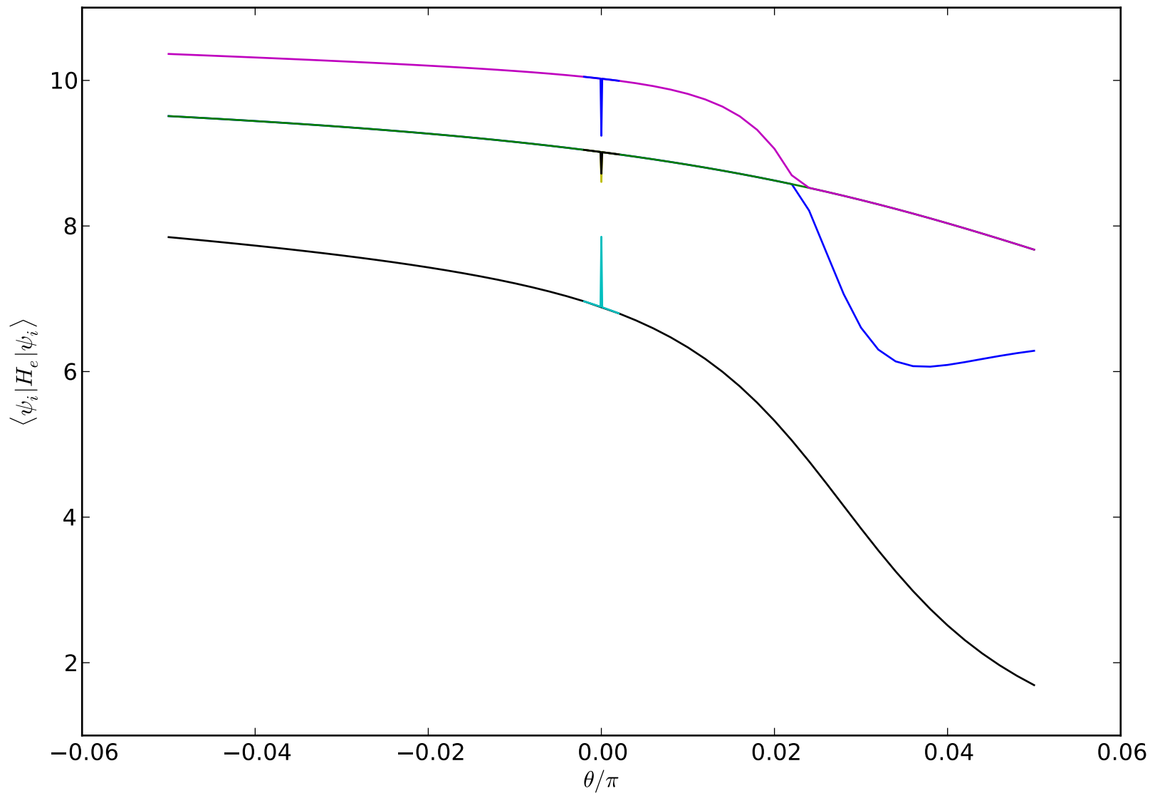
Projector model on 2x2 honeycomb: string tension
