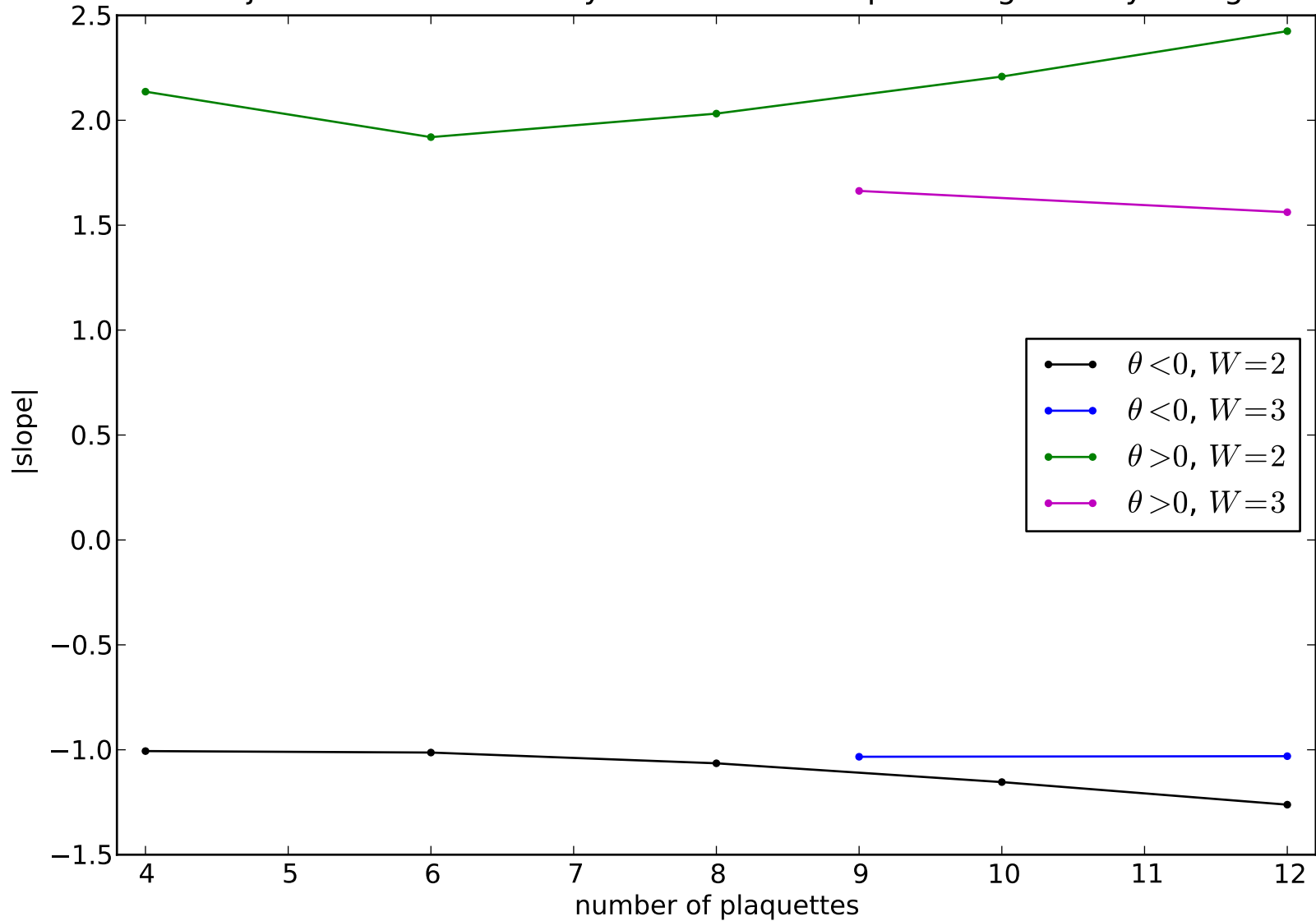
Projector model on honeycomb lattice: Slope of degeneracy lifting
