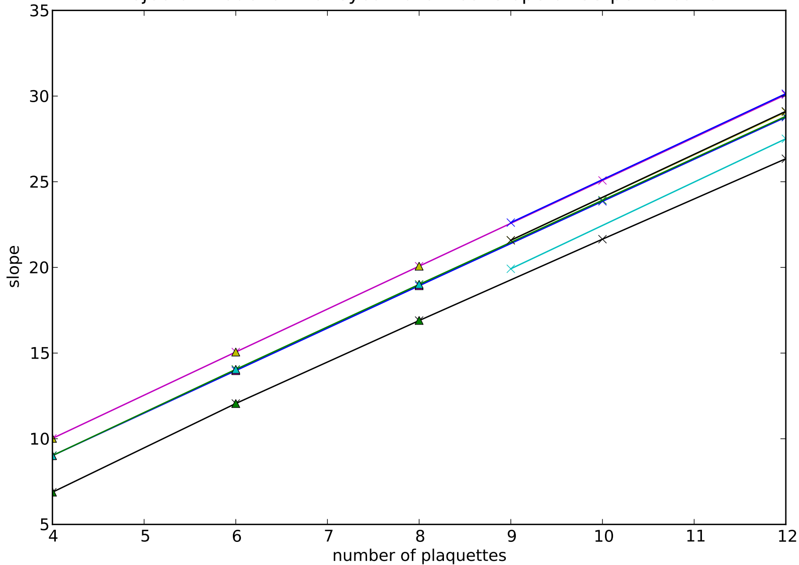
Projector model on honeycomb lattice: Slope of GS perturbation
