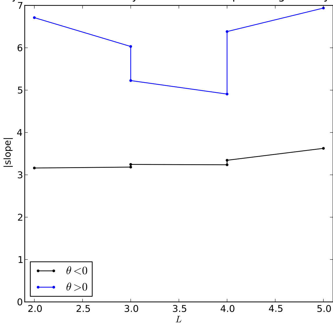
Projector model on honeycomb lattice: Slope of degeneracy lifting
