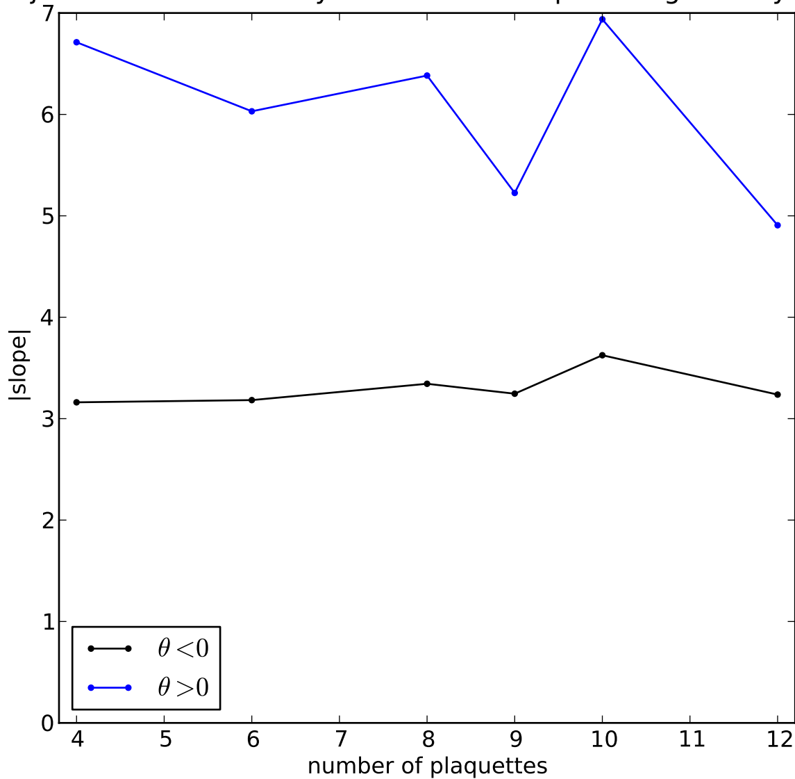
Projector model on honeycomb lattice: Slope of degeneracy lifting
