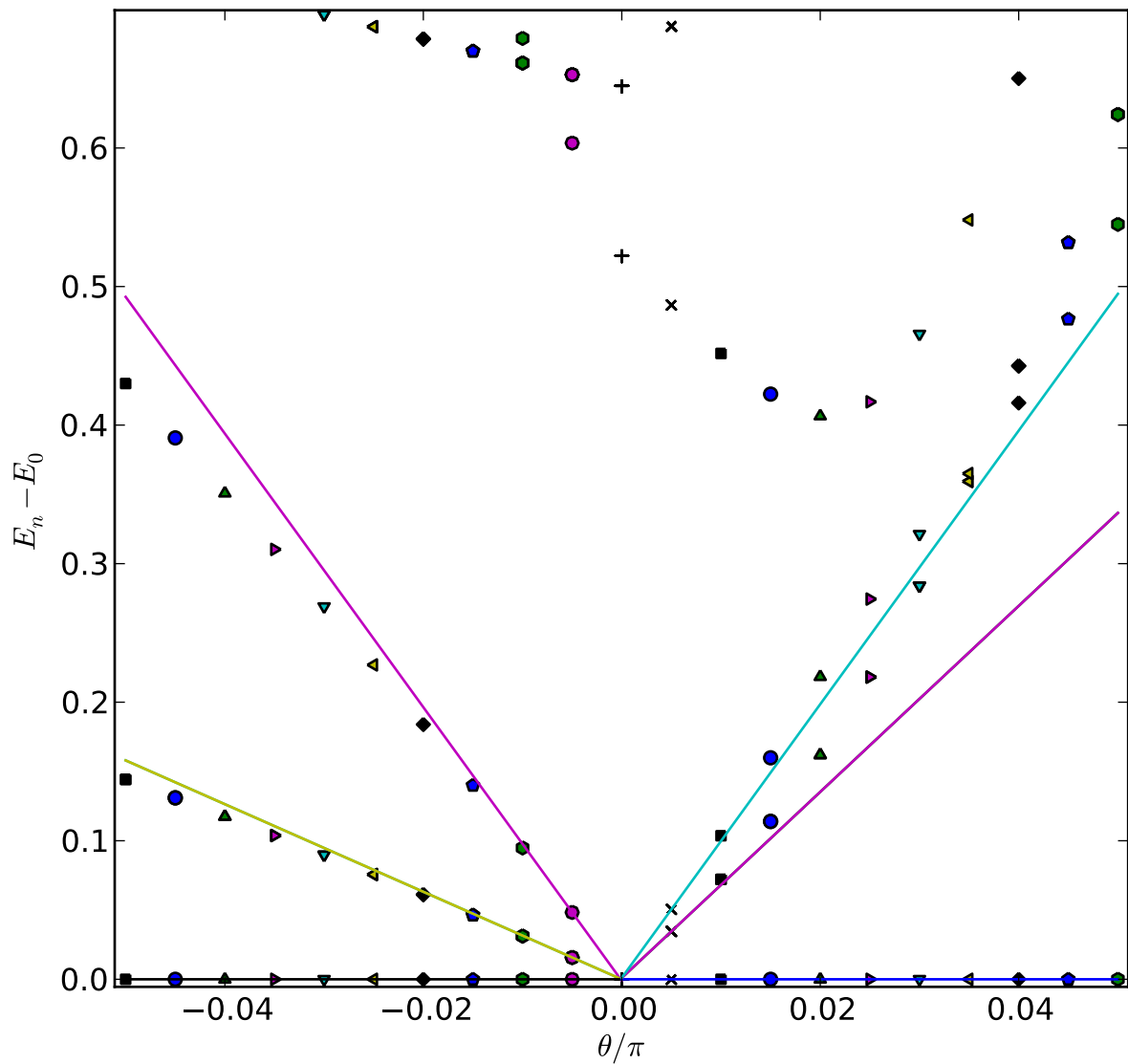
Projector model on 2x2 honeycomb lattice
