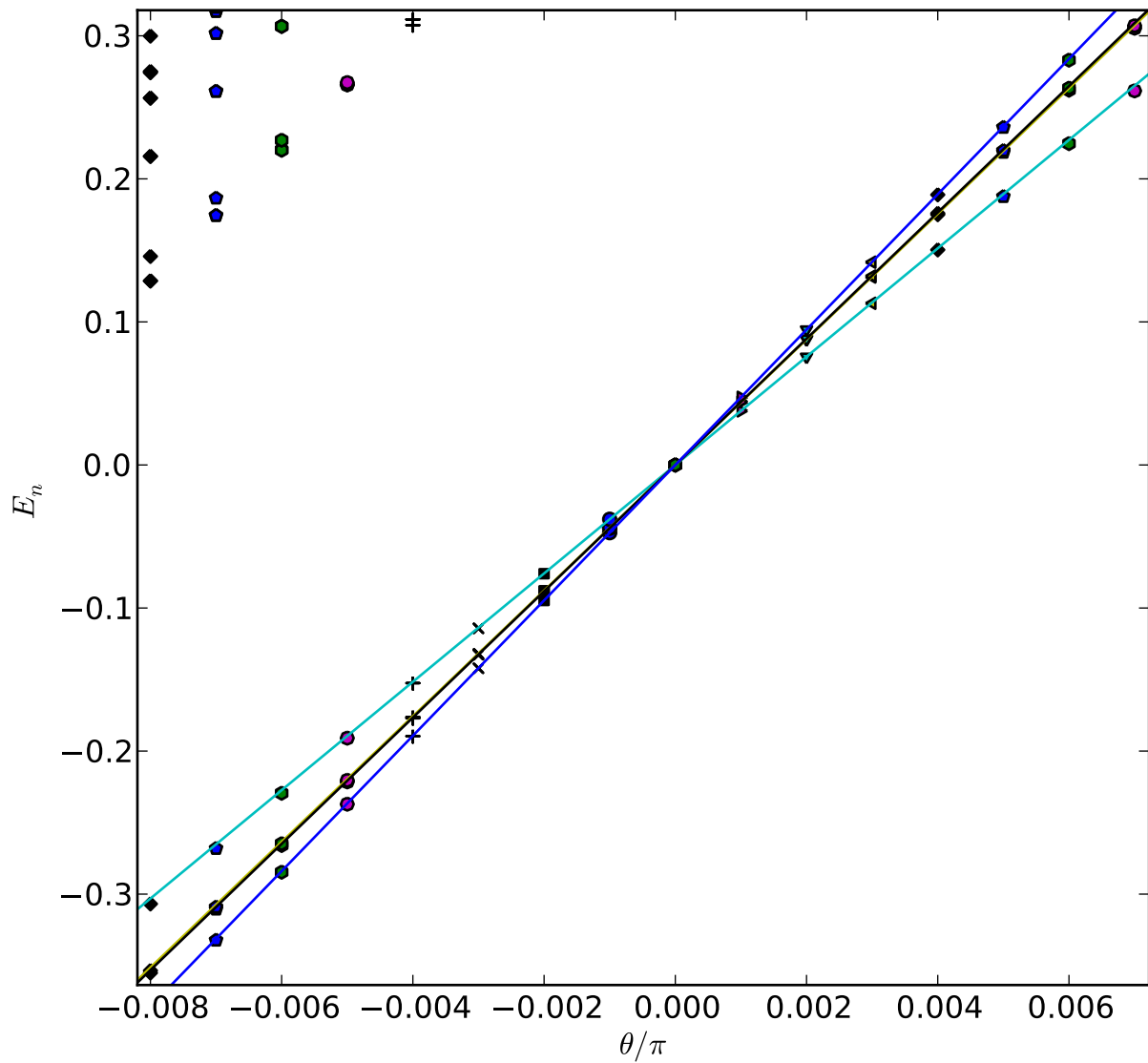
Projector model on 3x2 honeycomb lattice
