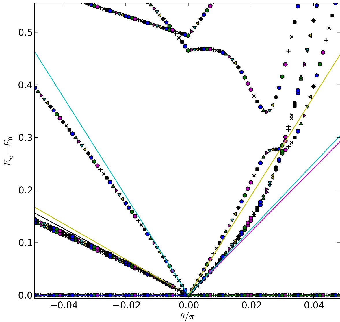
Projector model on 3x2 honeycomb lattice
