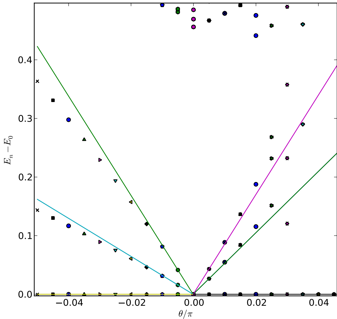
Spectrum of projector model on 3x3 honeycomb lattice
