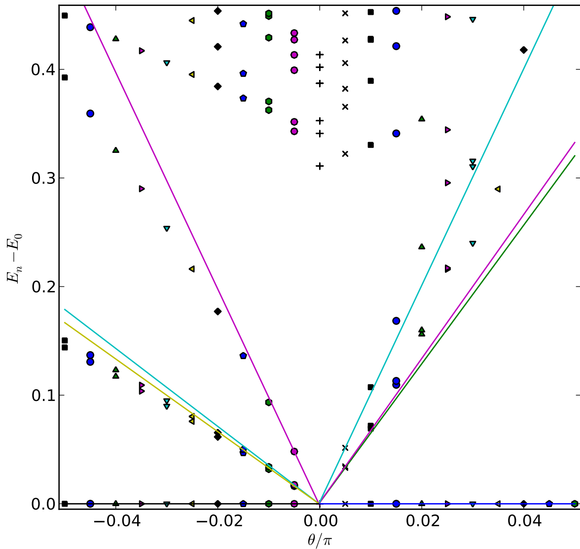
Projector model on 4x2 honeycomb lattice
