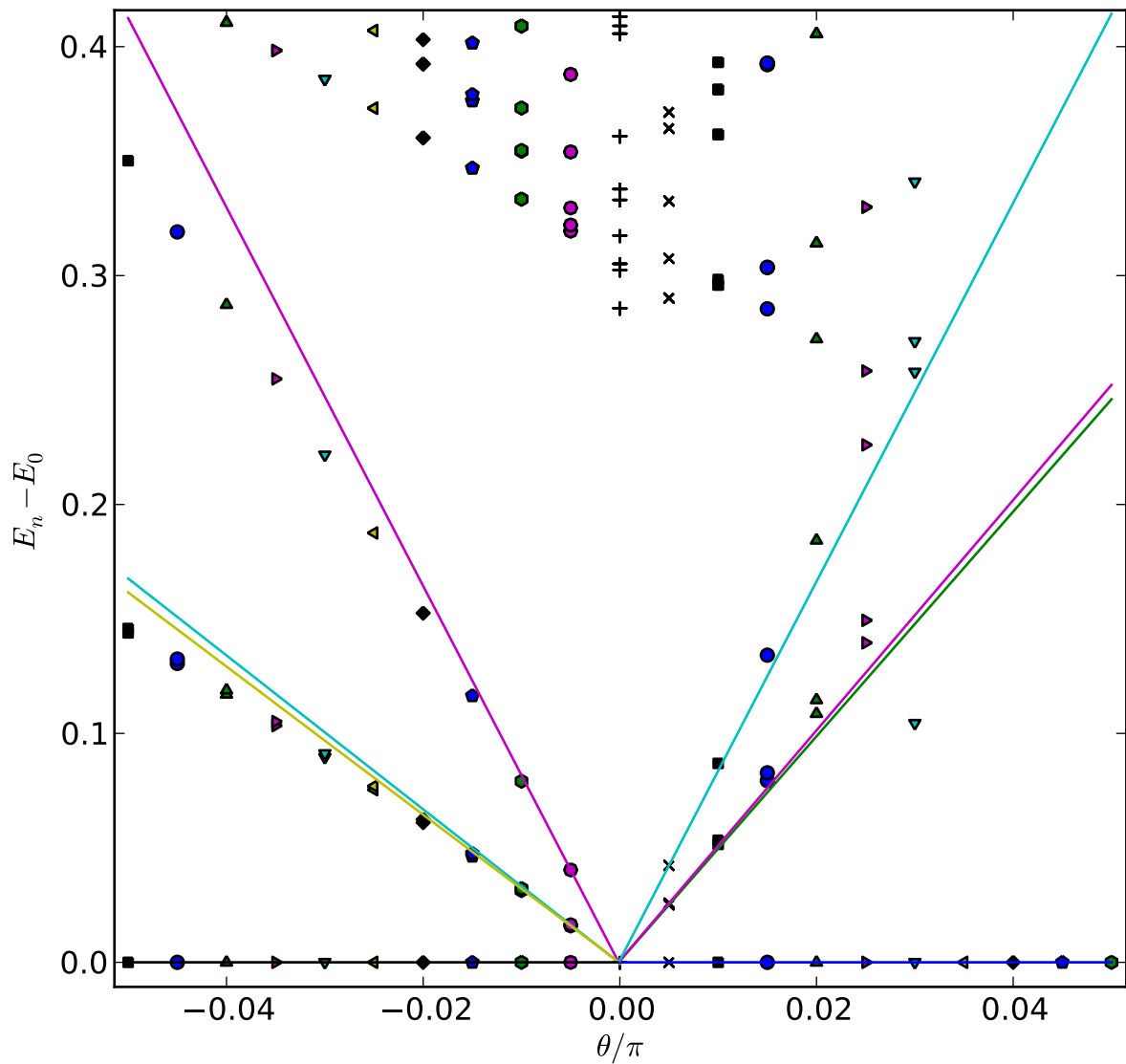
Projector model on 4x3 honeycomb lattice
