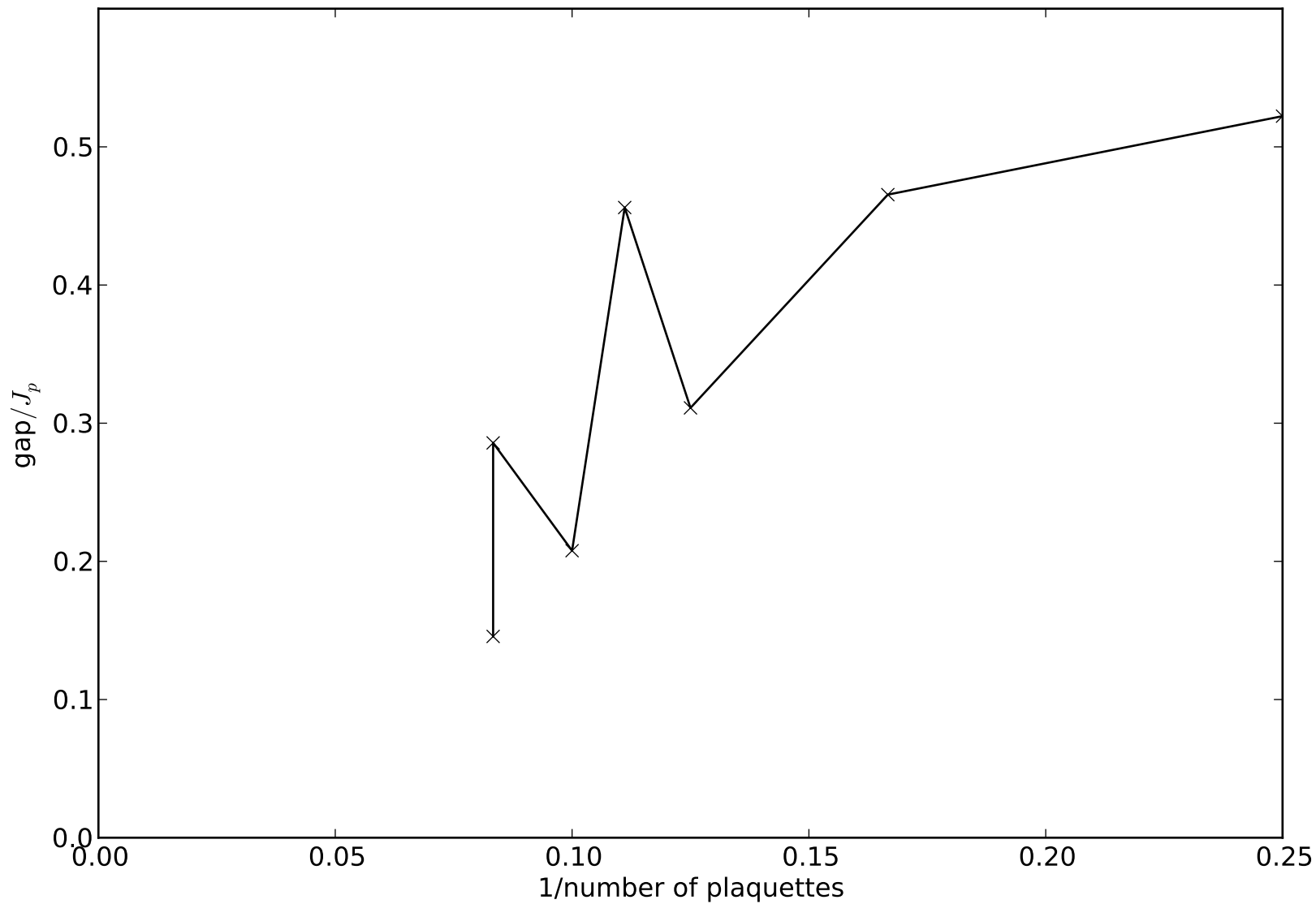
Projector model on honeycomb J_e = 0 : Scaling of the gap
