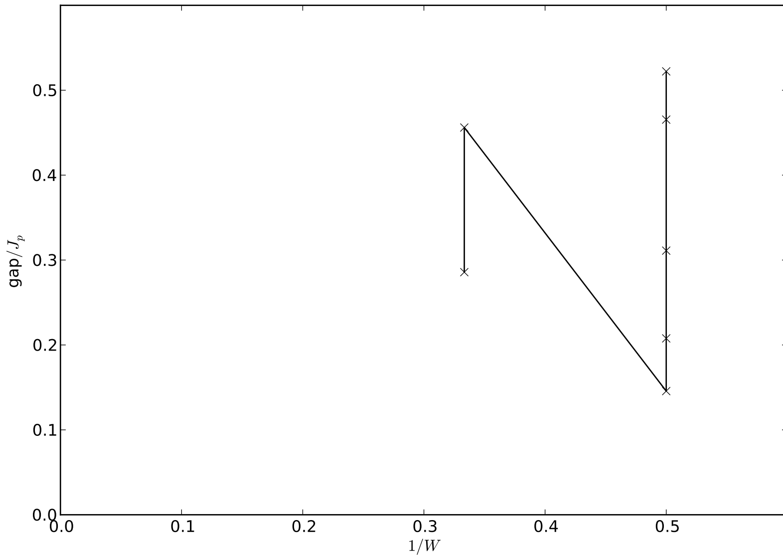
Projector model on honeycomb J_e = 0 : Scaling of the gap
