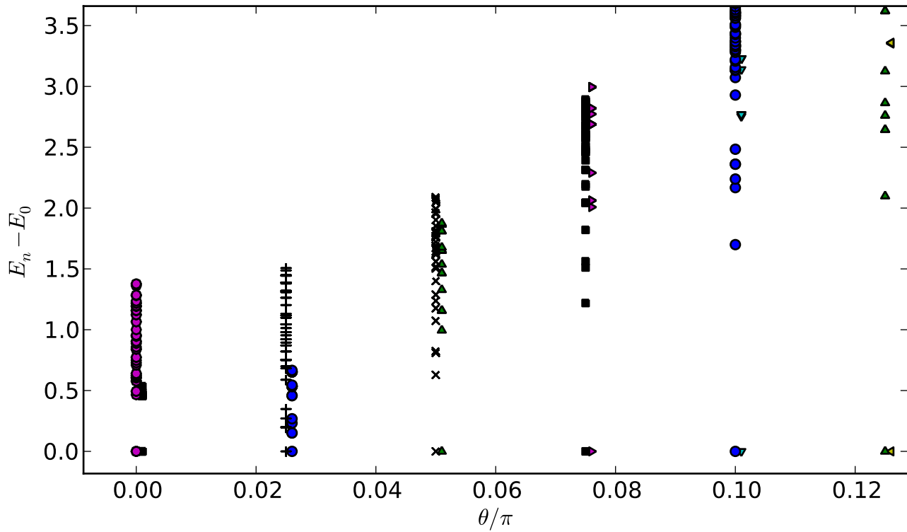
Spectrum of projector model on 3x2 honeycomb lattice
