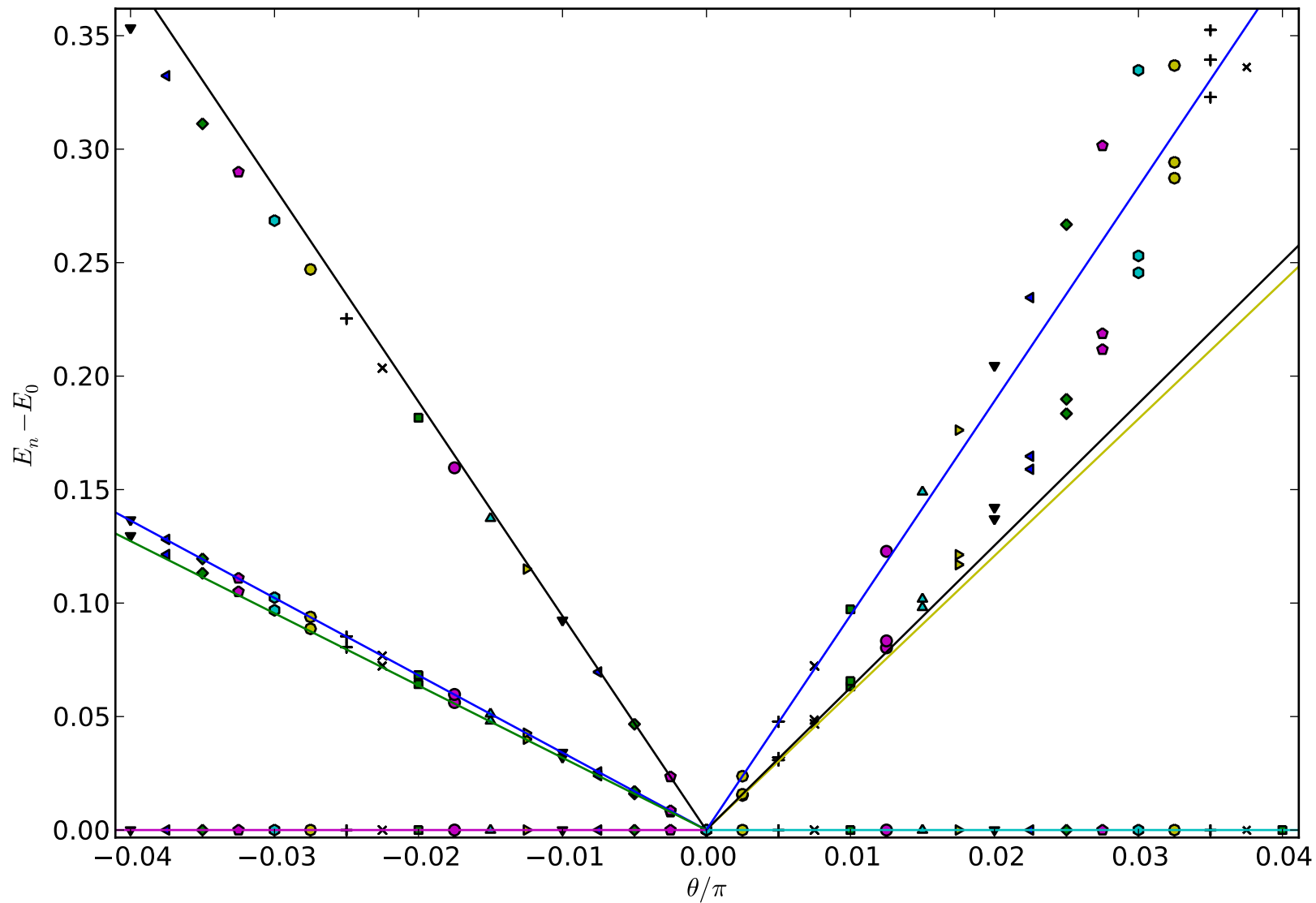
P^\dagger P model on 3x2 honeycomb lattice
