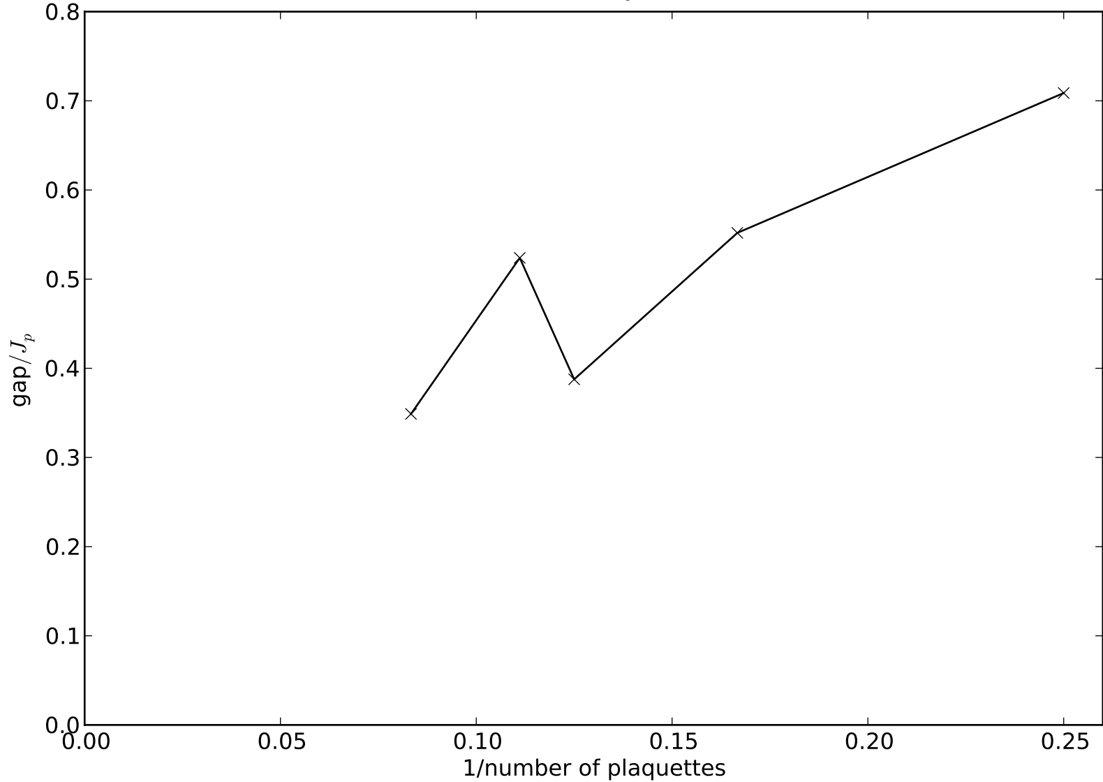
P^\dagger P model on honeycomb J_e = 0 : Scaling of the gap
