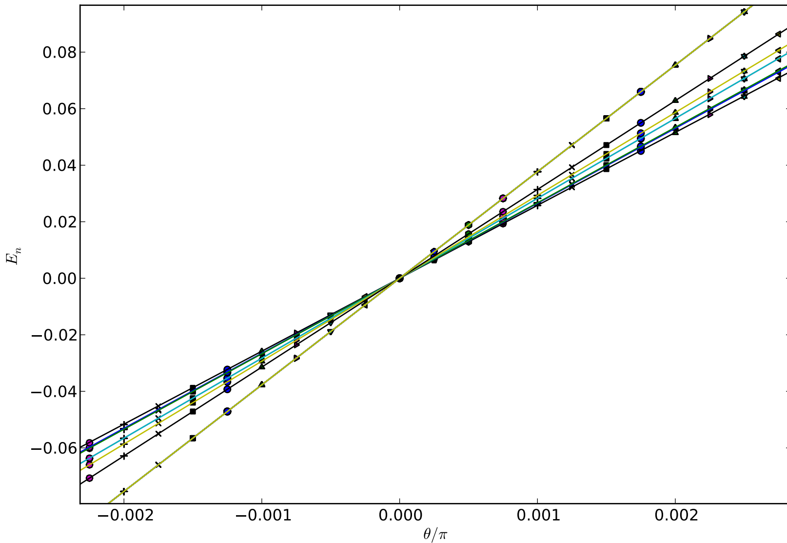
Gapless loop gas on 3x2 honeycomb lattice: magnetic field perturbation
