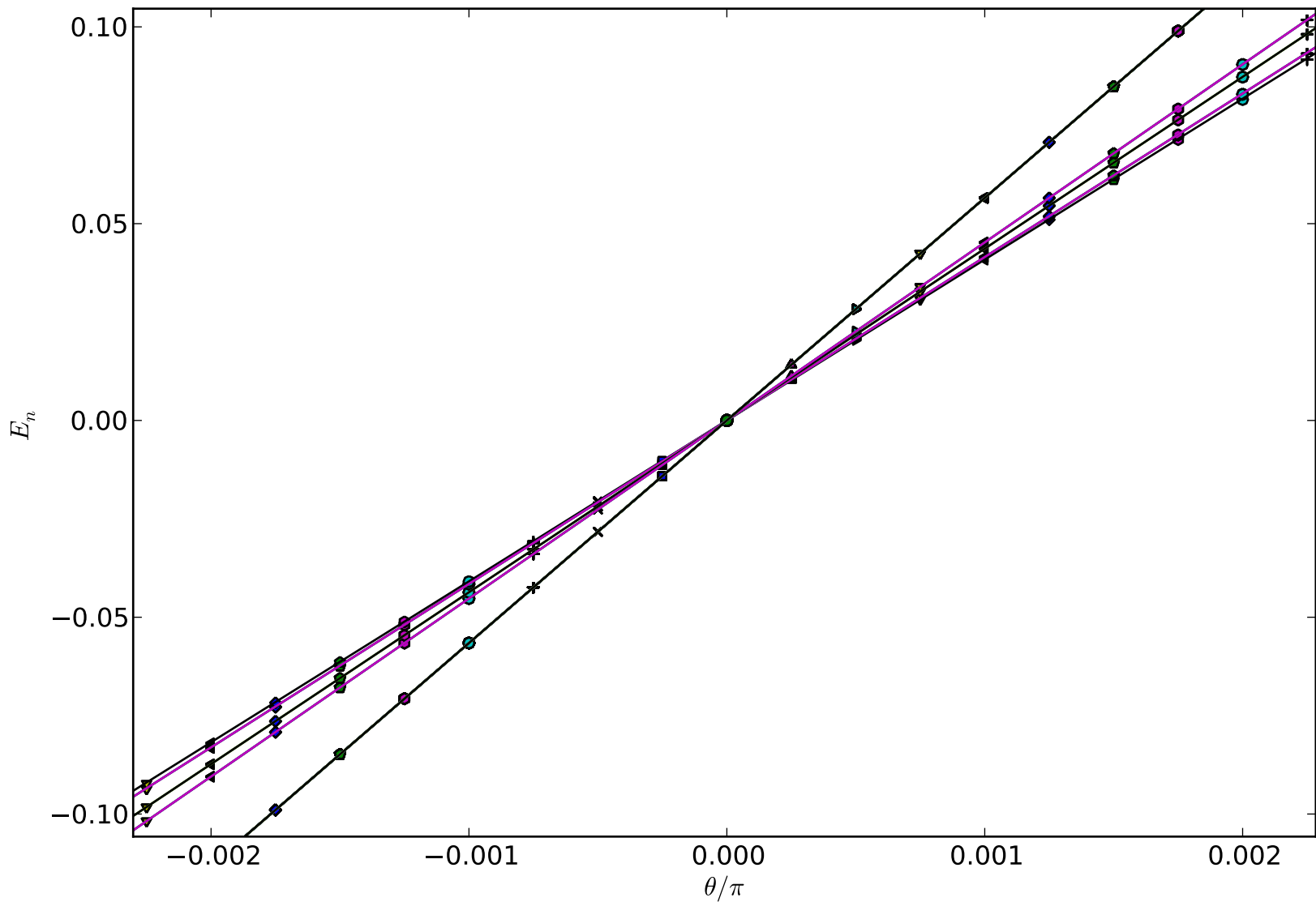
Gapless loop gas on 3x3 honeycomb lattice: magnetic field perturbation
