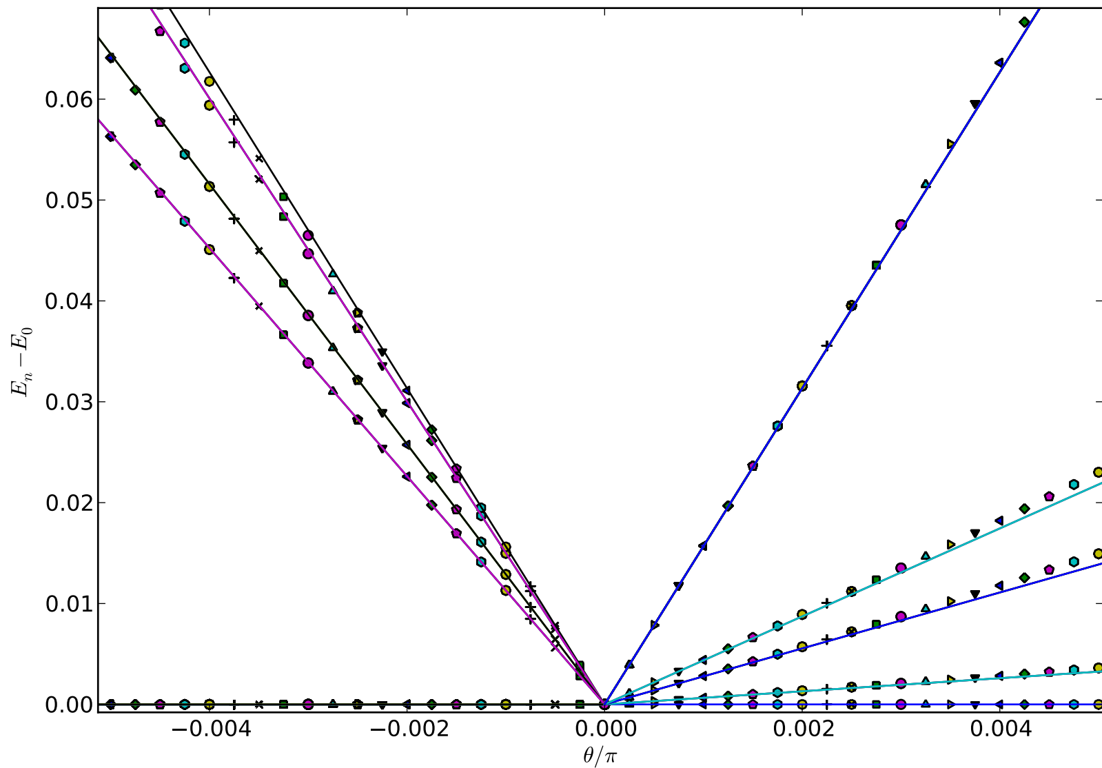
Gapless loop gas on 3x3 honeycomb lattice: magnetic field perturbation
