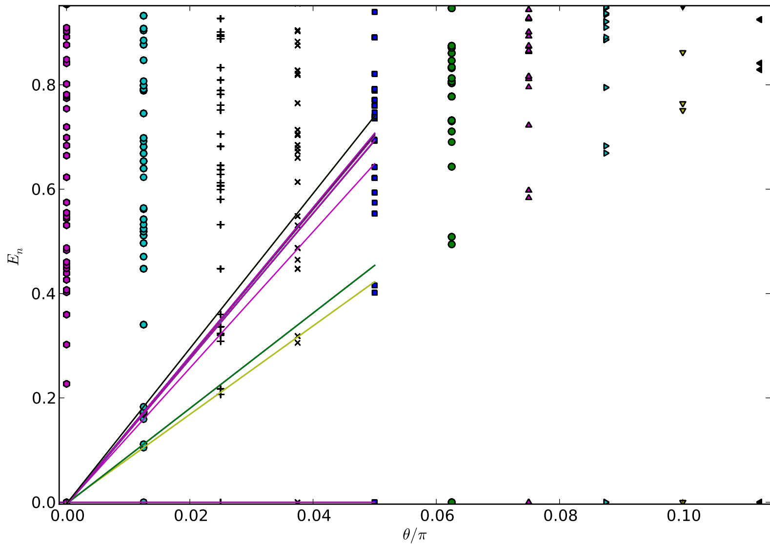
Gapless loop gas on 3x3 honeycomb lattice: surgery term perturbation
