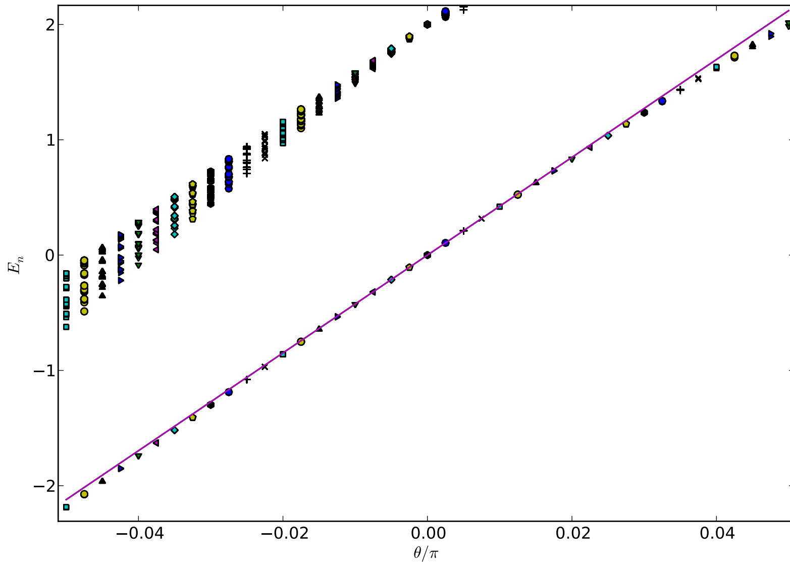
Toric code on 3x3 honeycomb lattice: magnetic field perturbation
