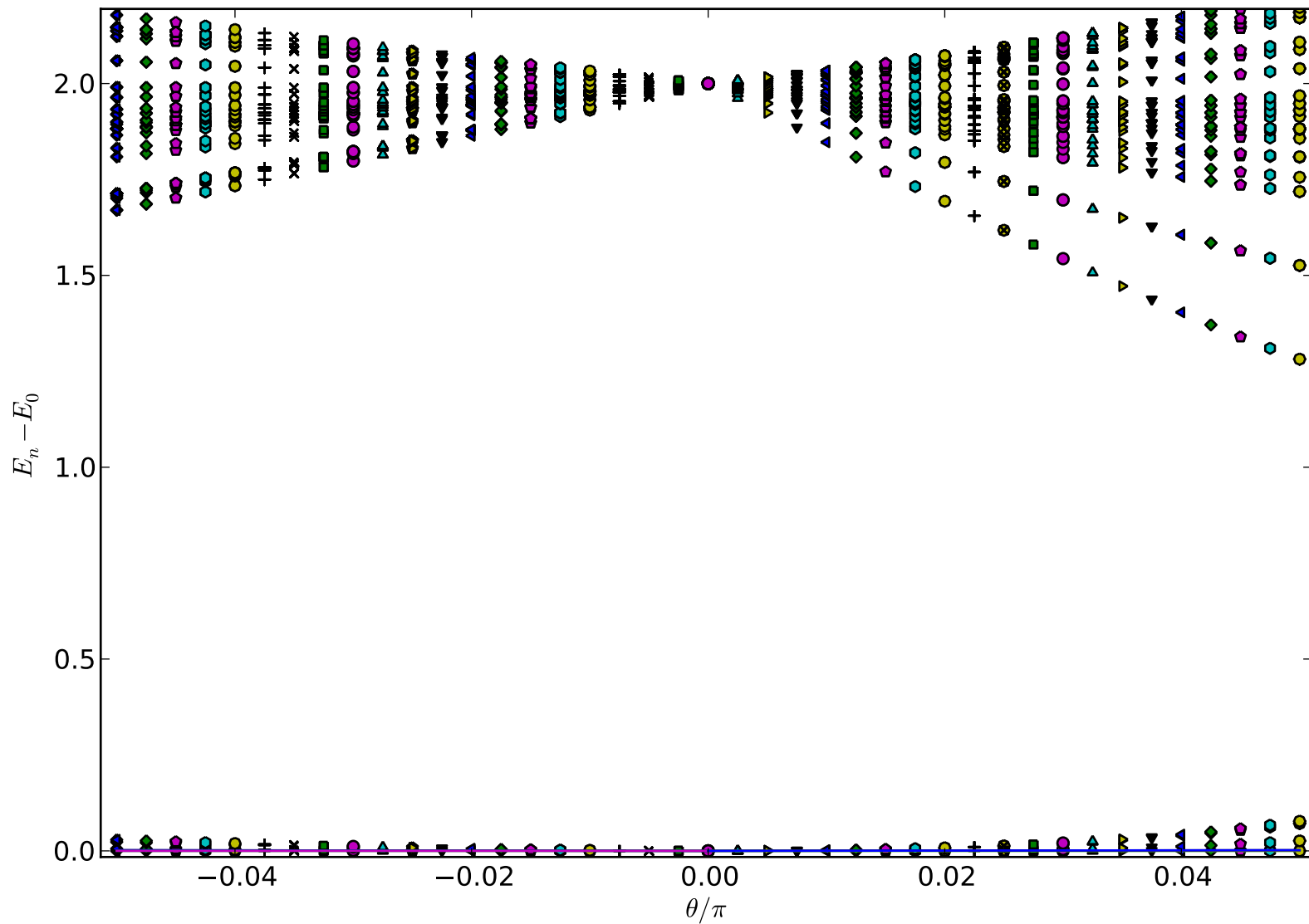
Toric code on 3x2 honeycomb lattice: magnetic field perturbation
