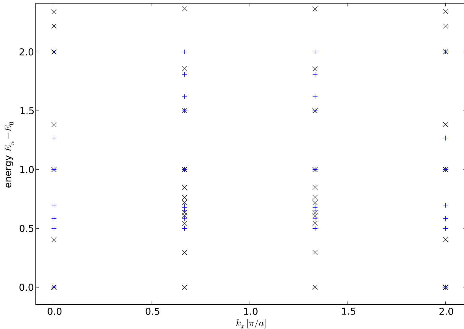
Spectrum: Gapless loop gas on 3x2 honeycomb lattice
