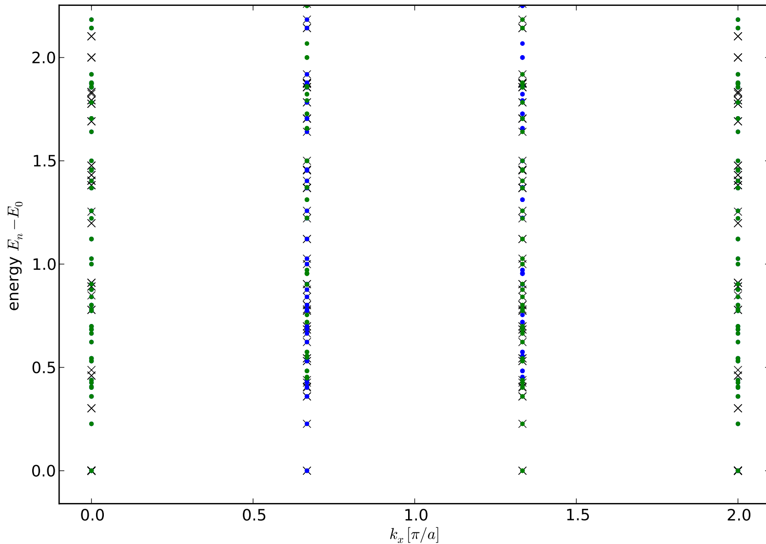
Spectrum: Gapless loop gas on 3x3 honeycomb lattice
