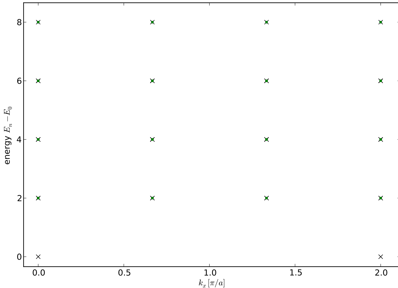
Spectrum: Toric code on 3x3 honeycomb lattice
