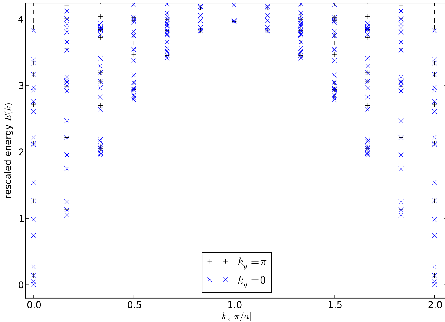
Spectrum: Fibonacci anyons on the ladder ( \theta = \frac{\pi}{4} , L=12 )
