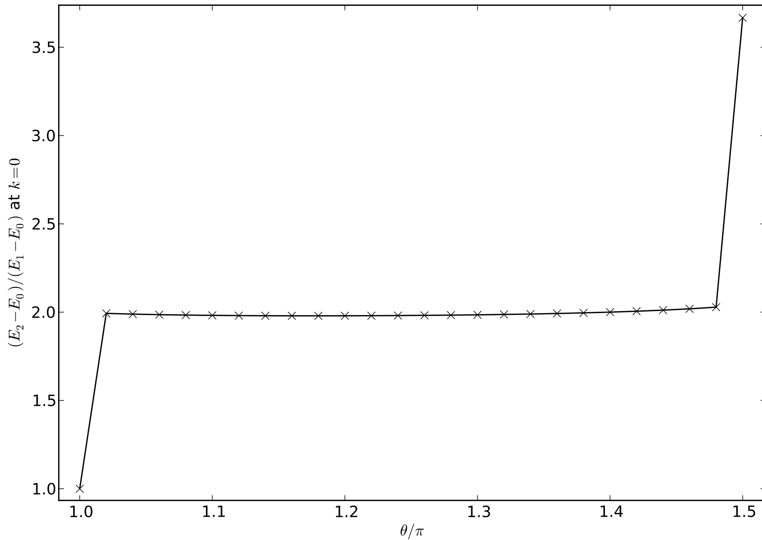
Fibonacci anyons on 10-rung ladder
