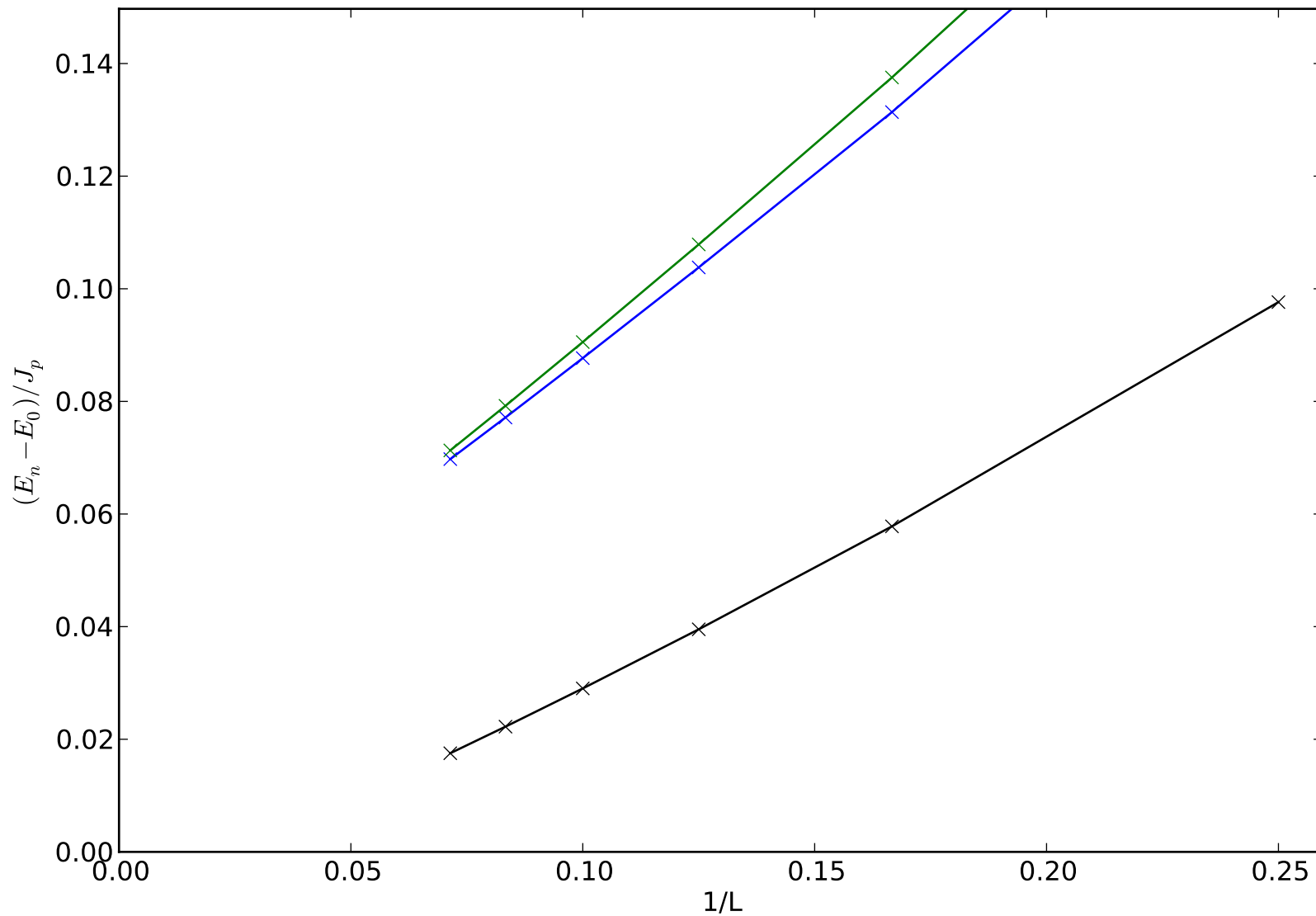
Fibonacci anyons on ladder J_e < 1, J_p \rightarrow 0^+ : Scaling of lowest states
