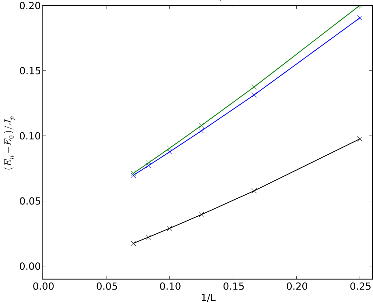
Fibonacci anyons on ladder J_e < 1, J_p \rightarrow 0^+ : Scaling of lowest states
