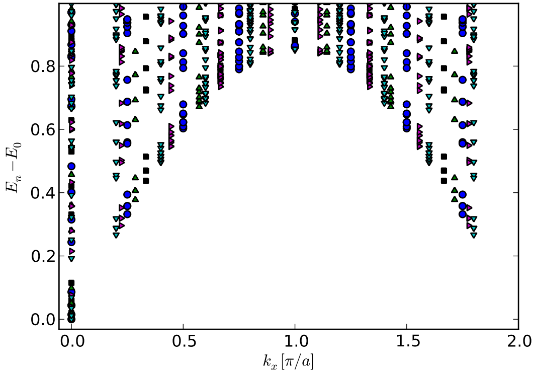
Spectrum: Fibonacci anyons on the ladder ( J_e/J_p=1 )
