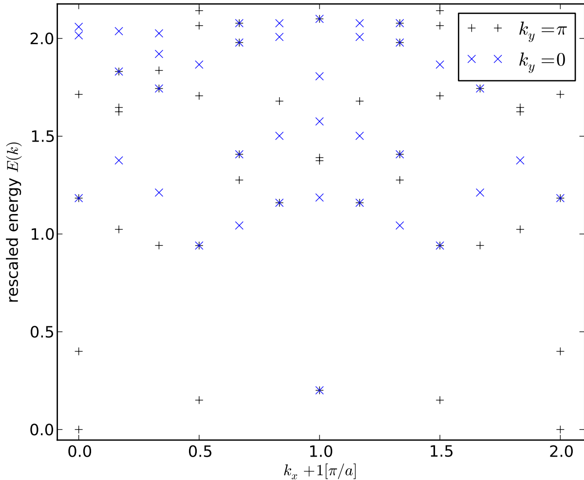
Spectrum: Fibonacci anyons on the ladder ( \theta \rightarrow \frac{3\pi}{2}^- , L=12 )
