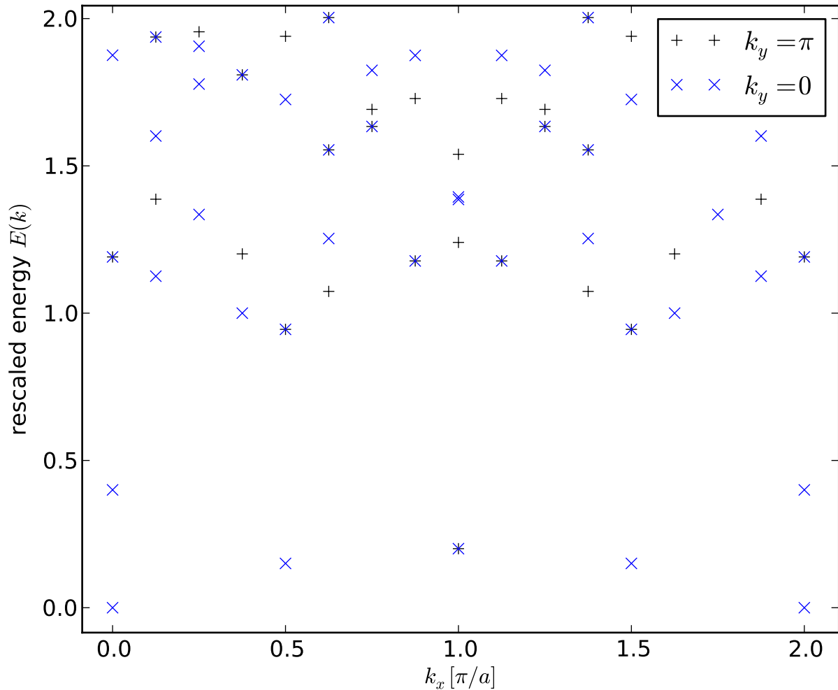
Spectrum: Fibonacci anyons on the ladder ( \theta \rightarrow \frac{3\pi}{2}^- , L=16 )
