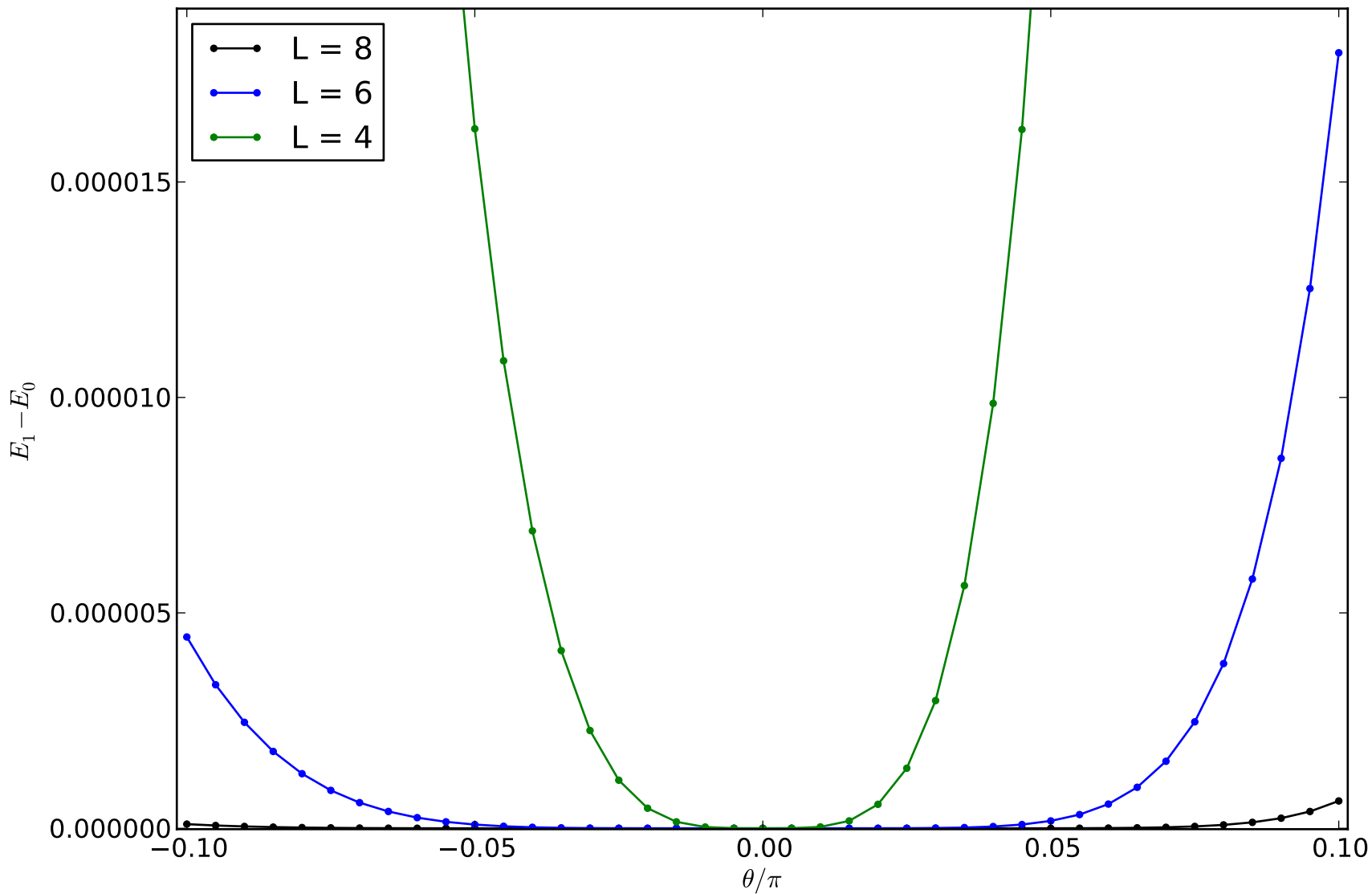
Fibonacci anyons on ladder: 1st excited state
