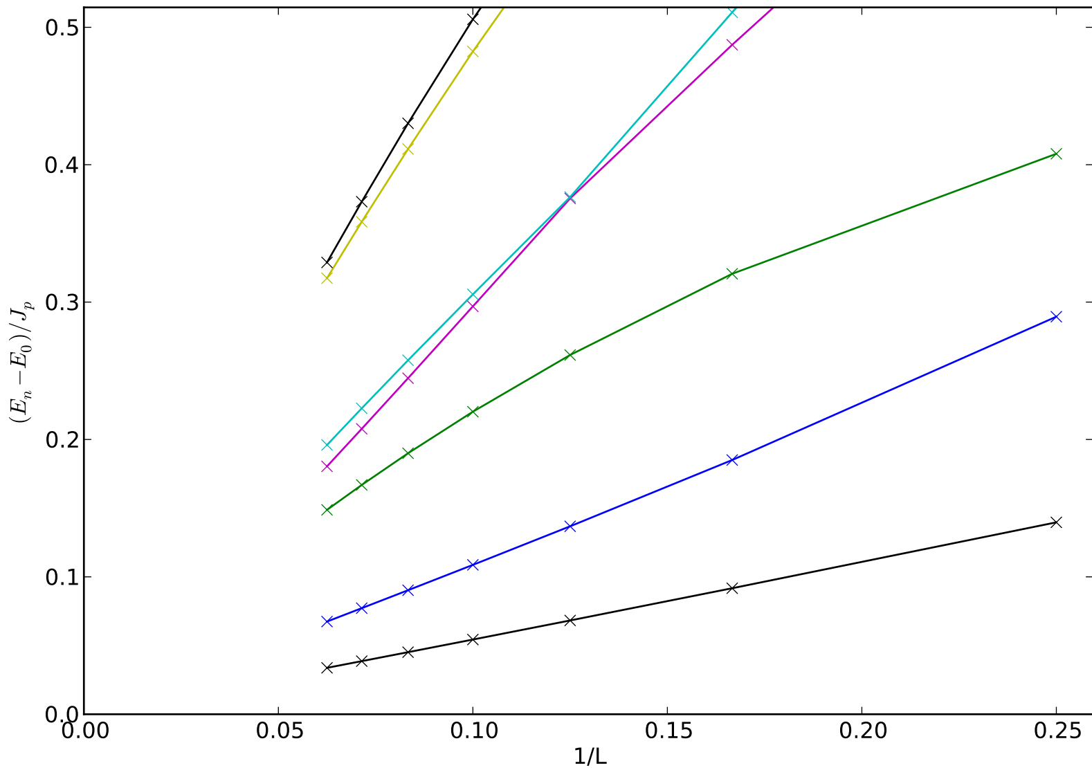
Galois conjugate on ladder J_e < 1, J_p \rightarrow 0^+ : Scaling of lowest states
