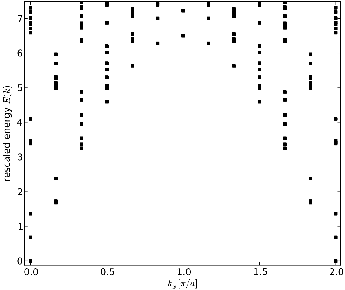
Spectrum: Galois conjugate on the ladder ( J_e = J_p < 0, L=12 )
