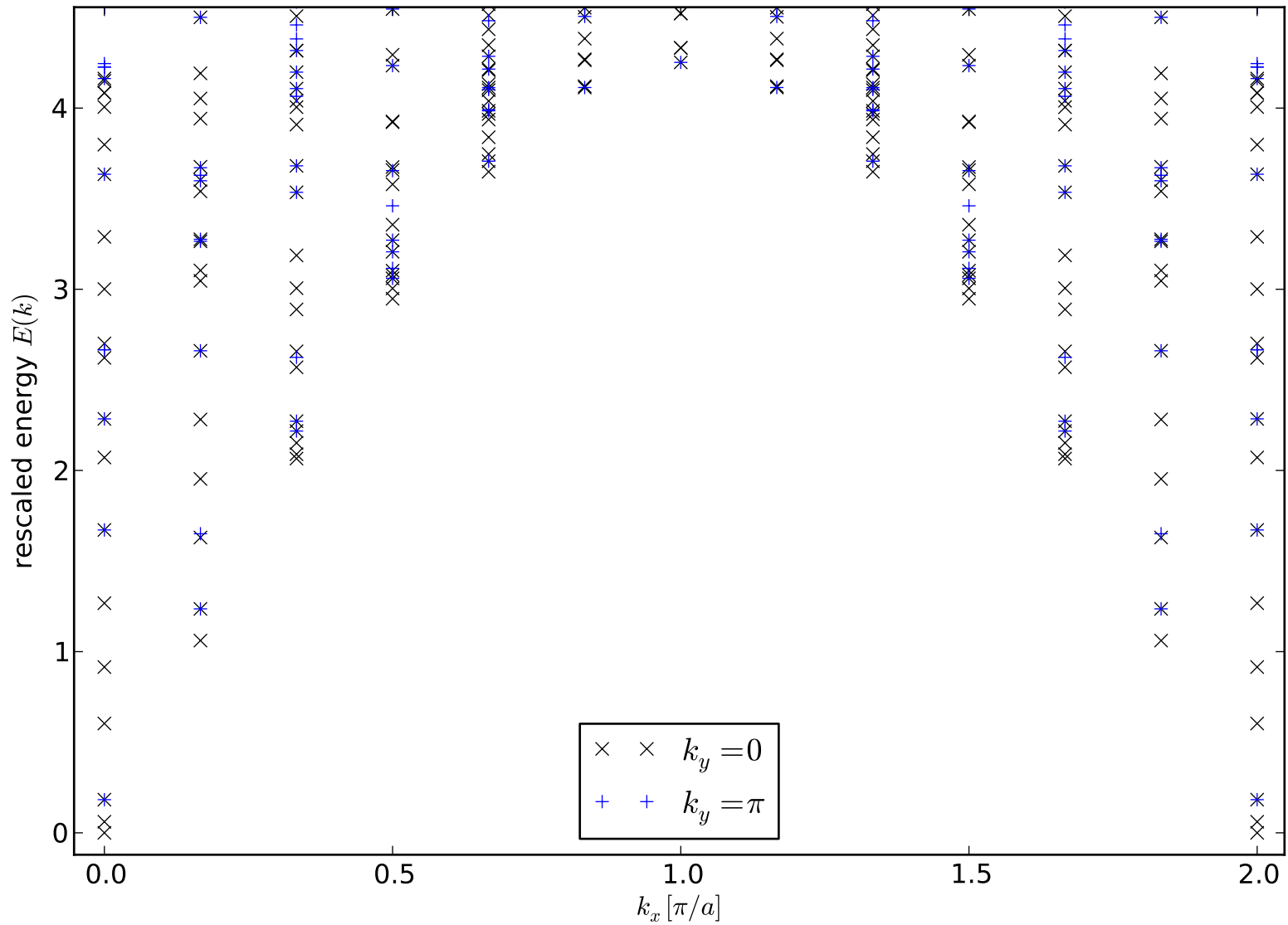
Spectrum: Galois conjugate on the ladder ( J_e = J_p = 1, L = 12 )
