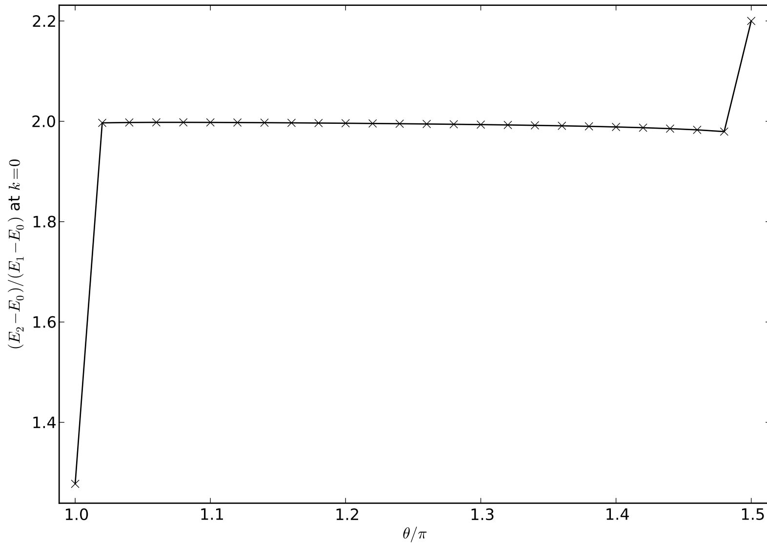
Galois conjugate on 10-rung ladder
