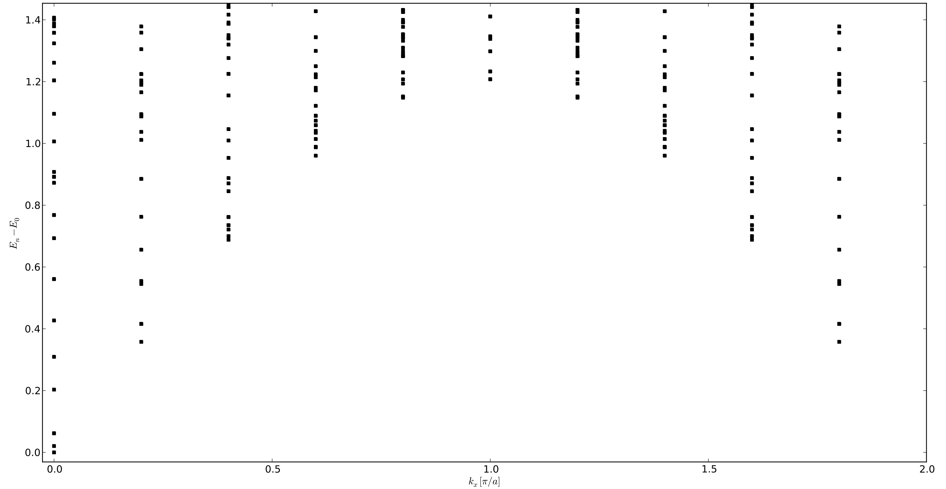
Spectrum: Galois conjugate on the ladder ( J_e/J_p = 1, L=10 )
