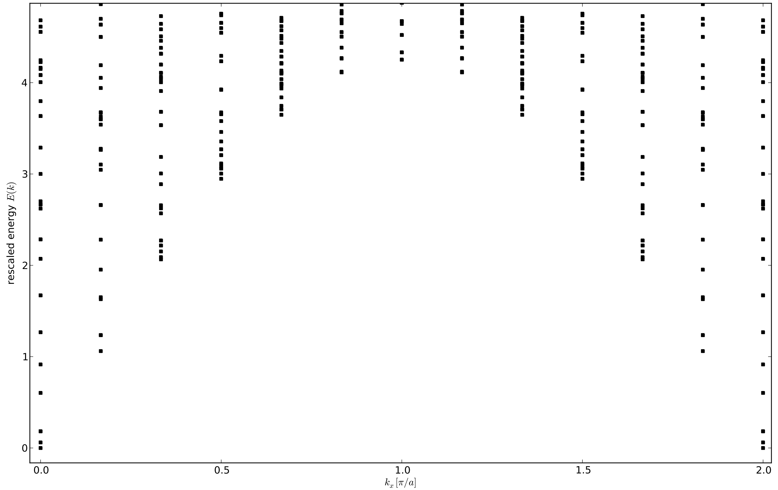
Spectrum: Galois conjugate on the ladder ( J_e/J_p = 1, L=12 )
