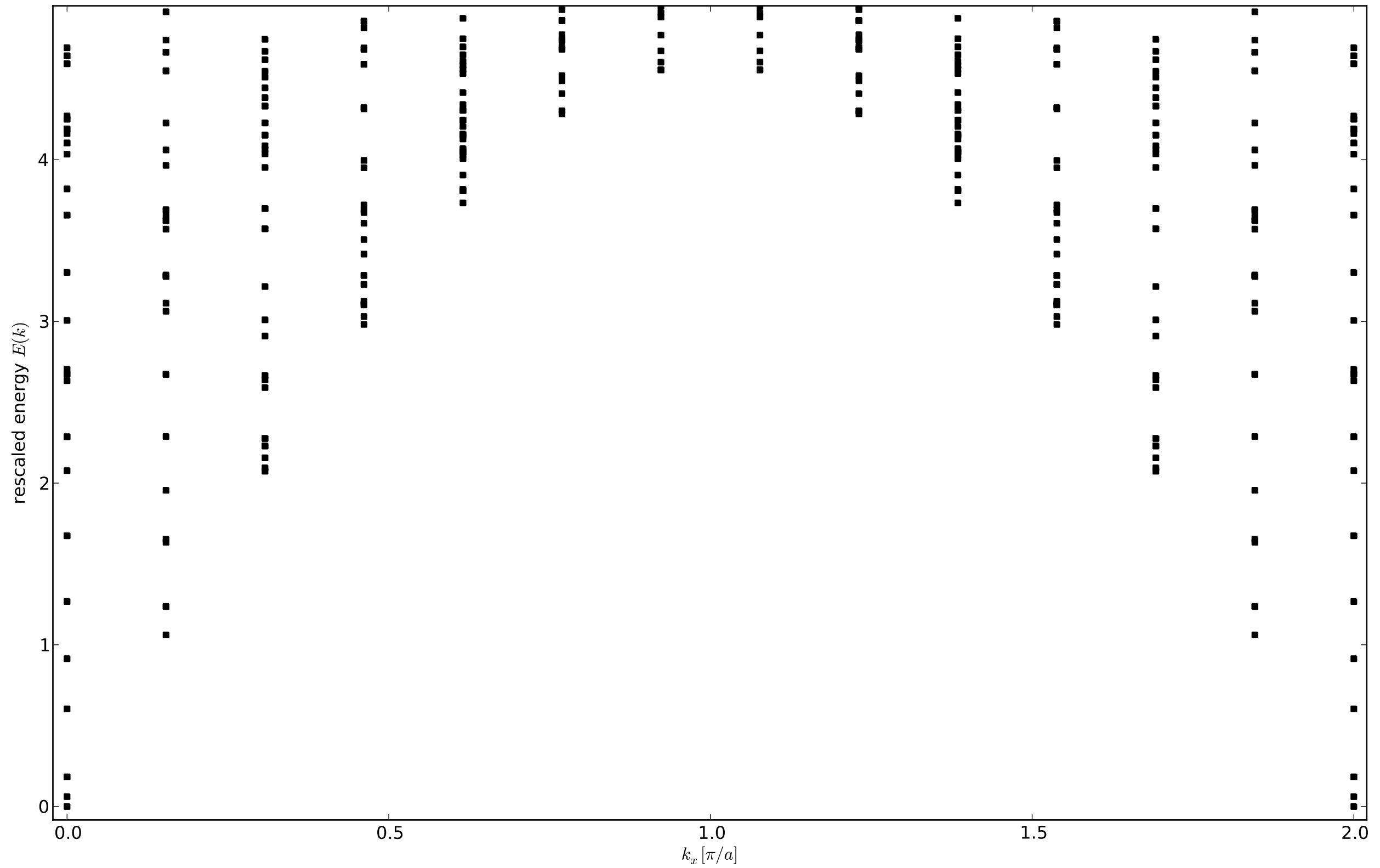
Spectrum: Galois conjugate on the ladder ( J_e/J_p = 1, L=13 )
