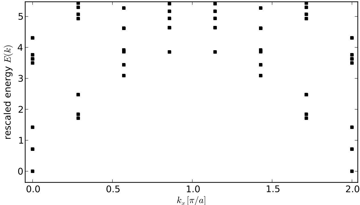
Spectrum: Galois conjugate on the ladder ( J_e = J_p < 0 , L=7 )
