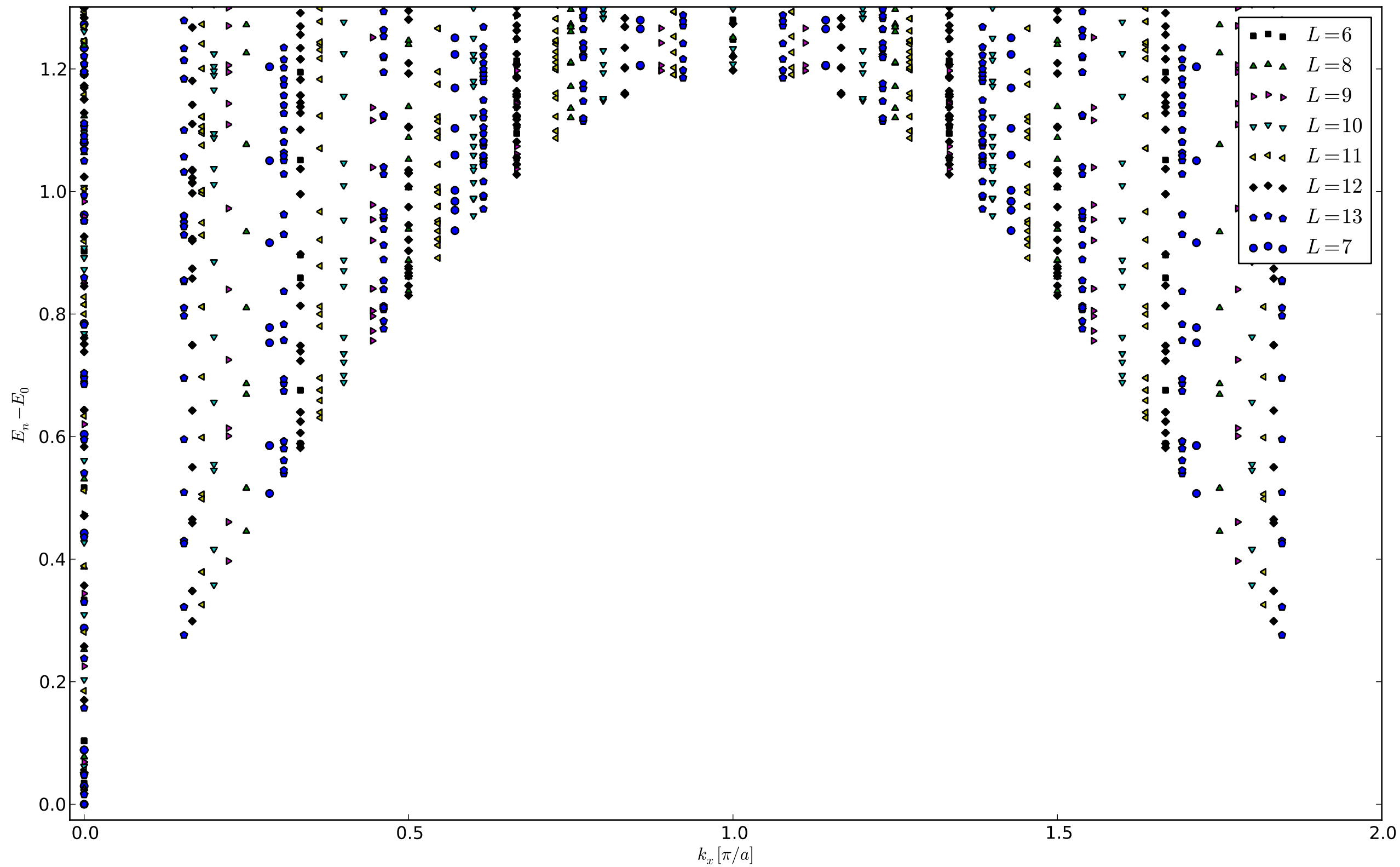
Spectrum: Galois conjugate on the ladder ( J_e/J_p = 1 )
